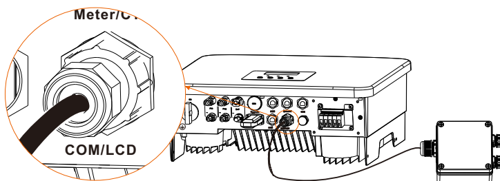
X1-Hybrid G4 inverter for an example
