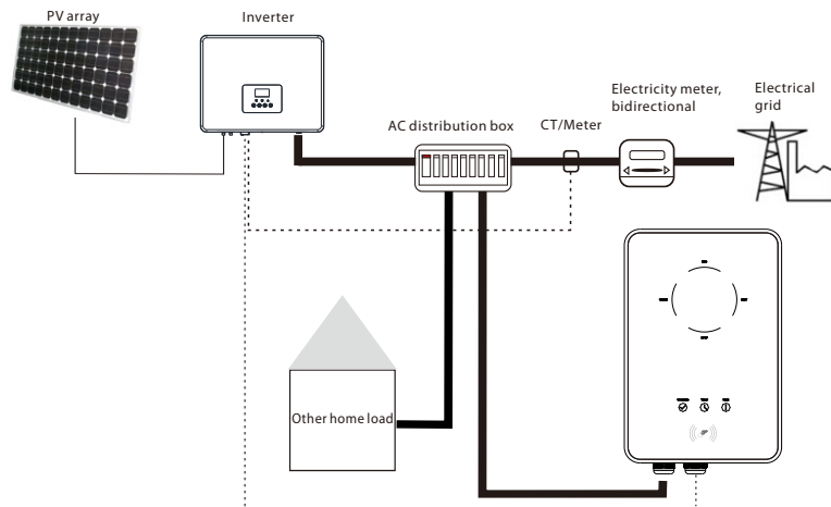
Communication with Inverter
