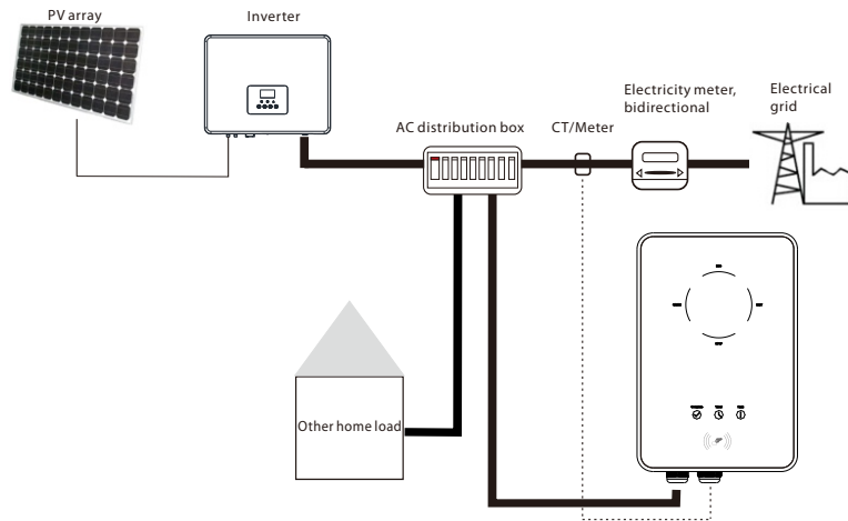
Communication with CT/Meter
